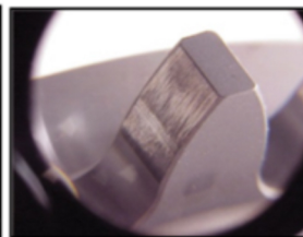
Scuffing
