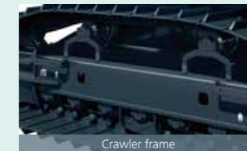
Crawler frame Special crawler frame design for easy mud removal cleaning.
